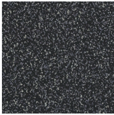
4623 Graphite Nebula
